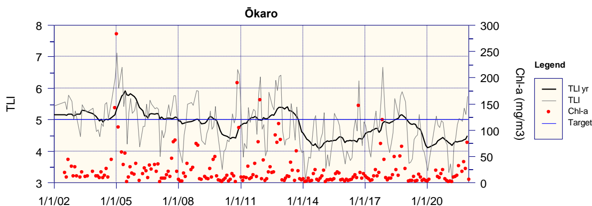
Figure 4.6 a: Rolling annual TLI compared the TLI target and monthly chlorophyll-a measurements in Lake Ōkaro, showing high values of chlorophyll-a (>60 mg/m 3 ) even when the annual TLI is below its target.
