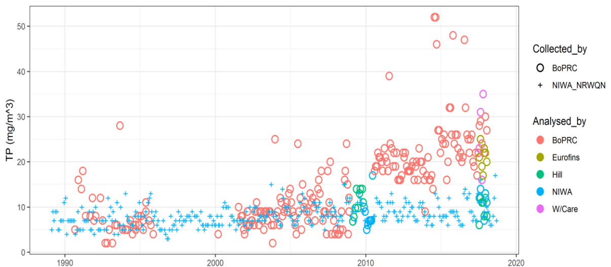
Figure B.3: TP in samples collected at Lake Tarawera outlet by NIWA NRWQN programme and Lake Tarawera mid-lake by BOPRC. Results of the inter-laboratory comparison in 2018 are also shown (from Baisden and McBride 2020).
