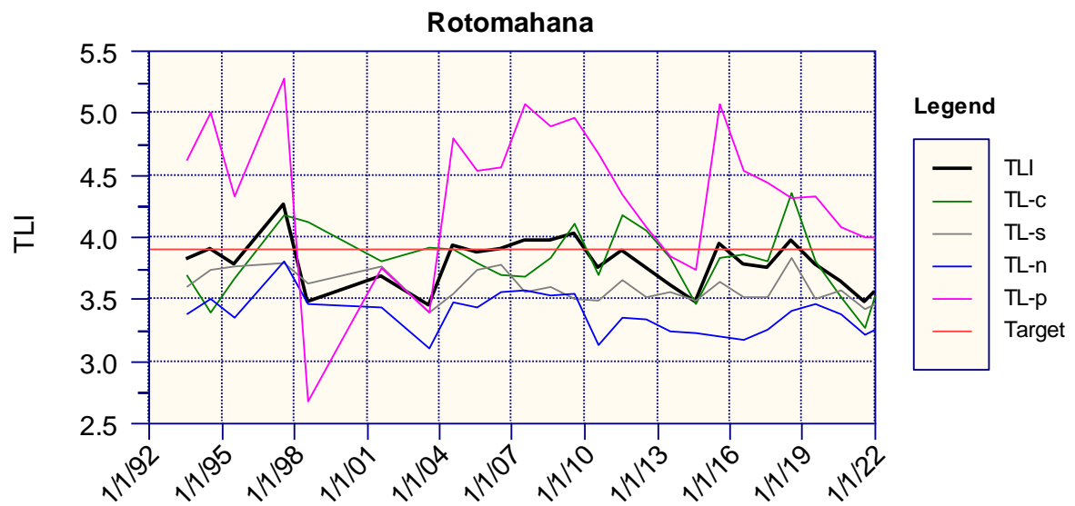
Figure 3.3 c: Annual mean TLI and targets. Dates are the end of the hydrological year.
