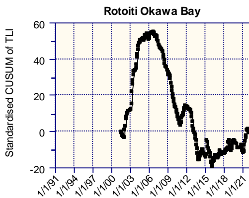
Figure E.1 b: Standardise CUSUM graphs for TLI. A straight line indicates no trend, an upward slope (A-shape) indicates an increasing trend, and a downward slope (U-shape) a decreasing trend.
