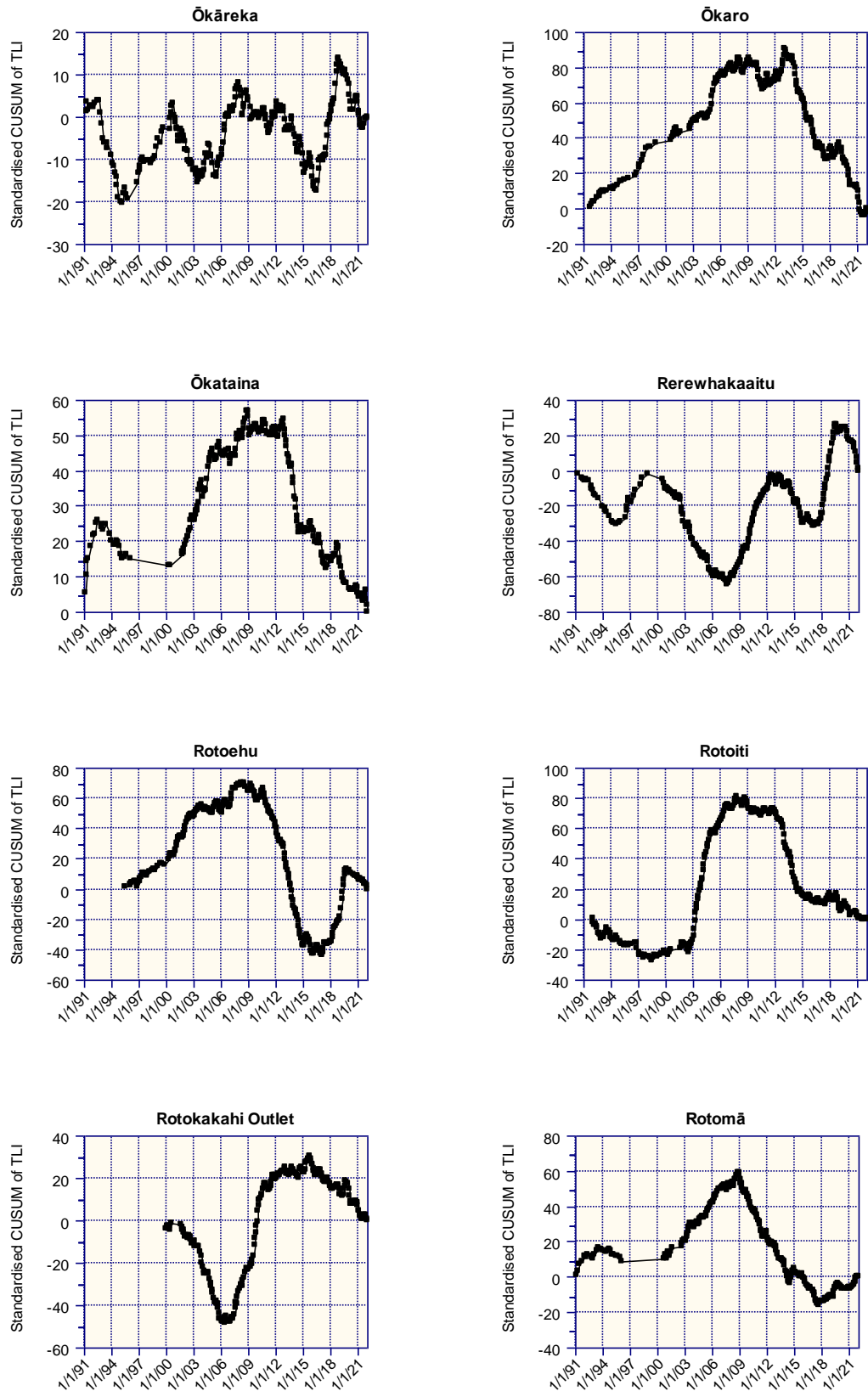
Figure E.1 a: Standardise CUSUM graphs for the TLI. A straight line indicates no trend, an upward slope (A-shape) indicates an increasing trend, and a downward slope (U-shape) a decreasing trend.
